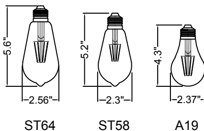
Recommended bulb shape
